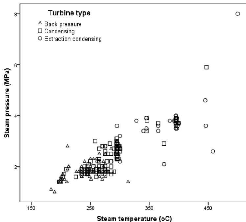
Figure 1. Distribution of Steam Condition and Turbine Type
