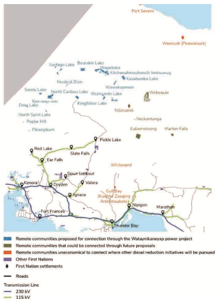
Figure 1. Watay Power Transmission Line Communities (Ontario Ministry Energy, 2017)
